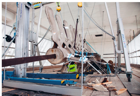
Figure 5. A large gantry was used to support the main armature while vertebrae were removed and cables were uncoupled.
