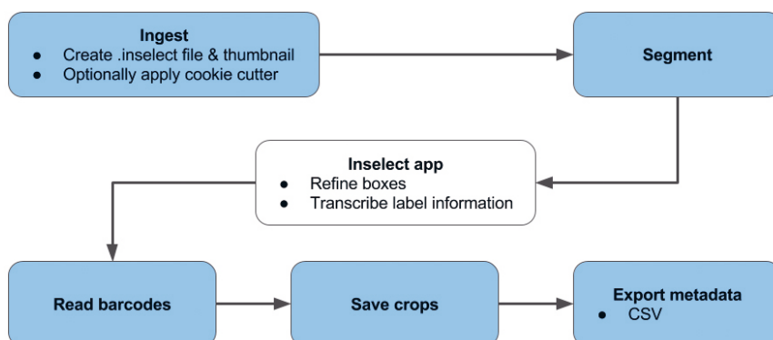
Figure 4. A typical Inselect workflow. Each of the blue boxes has a corresponding command-line tool that operates on batches of images.
