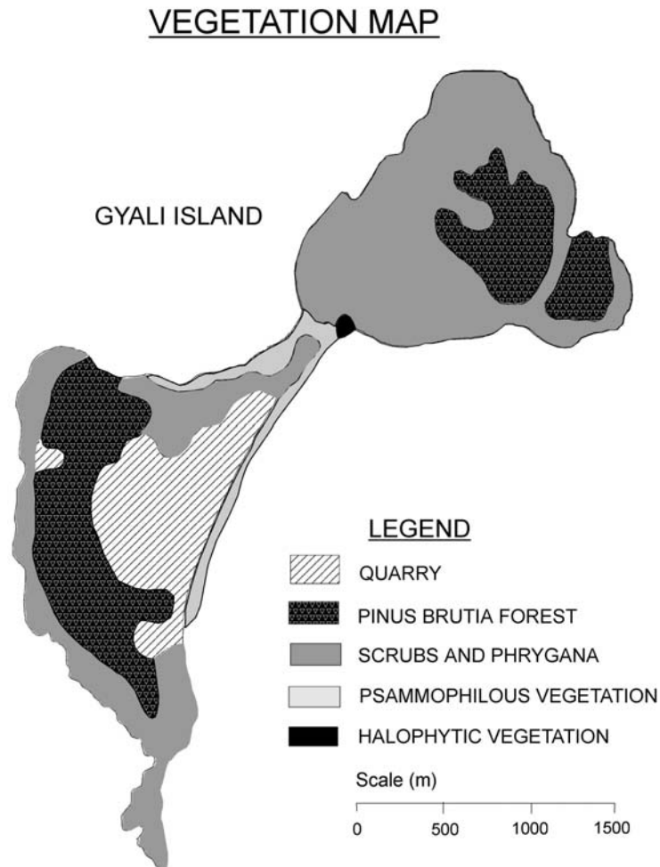
Fig. 3. Vegetation map of Gyali island.
