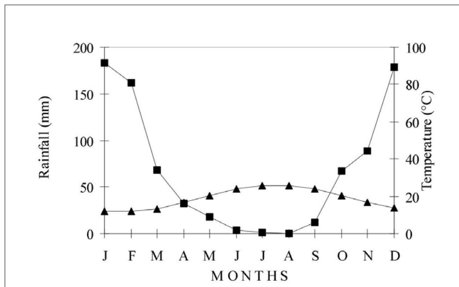
Fig. 2. Ombrothermic diagram of Kos meteorological station.
