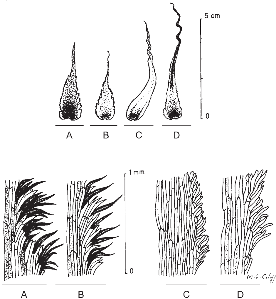
Fig. 2. Petiole scale (above), with enlarged portion of its margin (below), of A: Cyathea armata ; B: C. strigillosa ; C: C. arborea ; D: C. \times calolepis .
