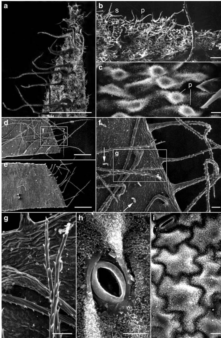
Fig. 3. Hieracium olympicum , scanning electron micrographs of involucre bracts (a-c) and basal leaves (d-i) – a-c: low, medium and high magnification of involucre bract surface, densely covered with stellate hairs (= s), short simple hairs and numerous epidermal papillae (= p) covered with rod-shaped and short filiform wax crystalloids; d-i: basal leaves with numerous microglands (arrows) on lower side (d, f, g, h) and upper side (e, i); cover with trabecular wax crystalloids and simple hairs with short teeth (denticuli) (f, g) and shortly forked or simple tips. – Scale bars: a, d, e = 1 mm; b, f, g = 100 \mu m; c, h, i = 10 \mu m; specimen: Turkey, 30.7.1988, M. Nydegger 43912 (herb. Gottschlich 9944, Soc. Éch. Pl. Vasc. Eur. Méd. 14620).
