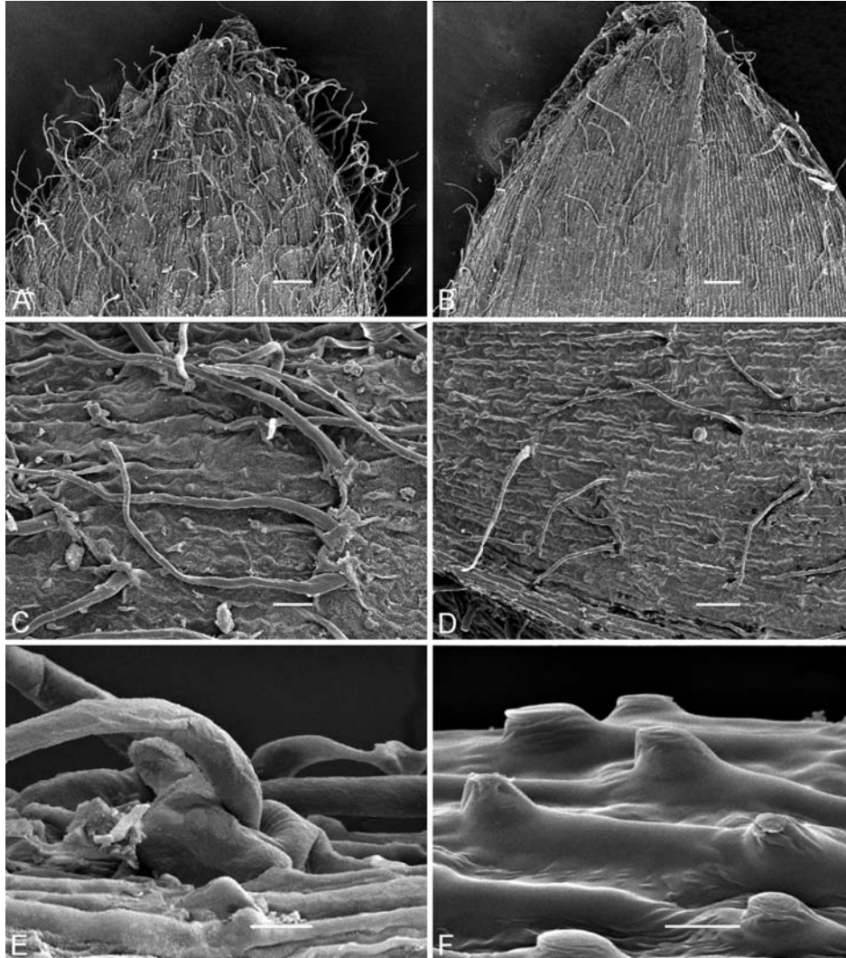
Fig. 2. Scanning electron micrographs. – A, C, E: Paspalum quadrifarium – spikelet tip (A); detail of hairs on upper glume (C); detail of bulbous-based hair (E); from F. Verloove 6004 . – B, D, F: P. exaltatum – spikelet tip (B); detail of hairs on upper glume (D); detail of silica bodies on the upper floret (F); from F. Garbari 23.9.1966 .
